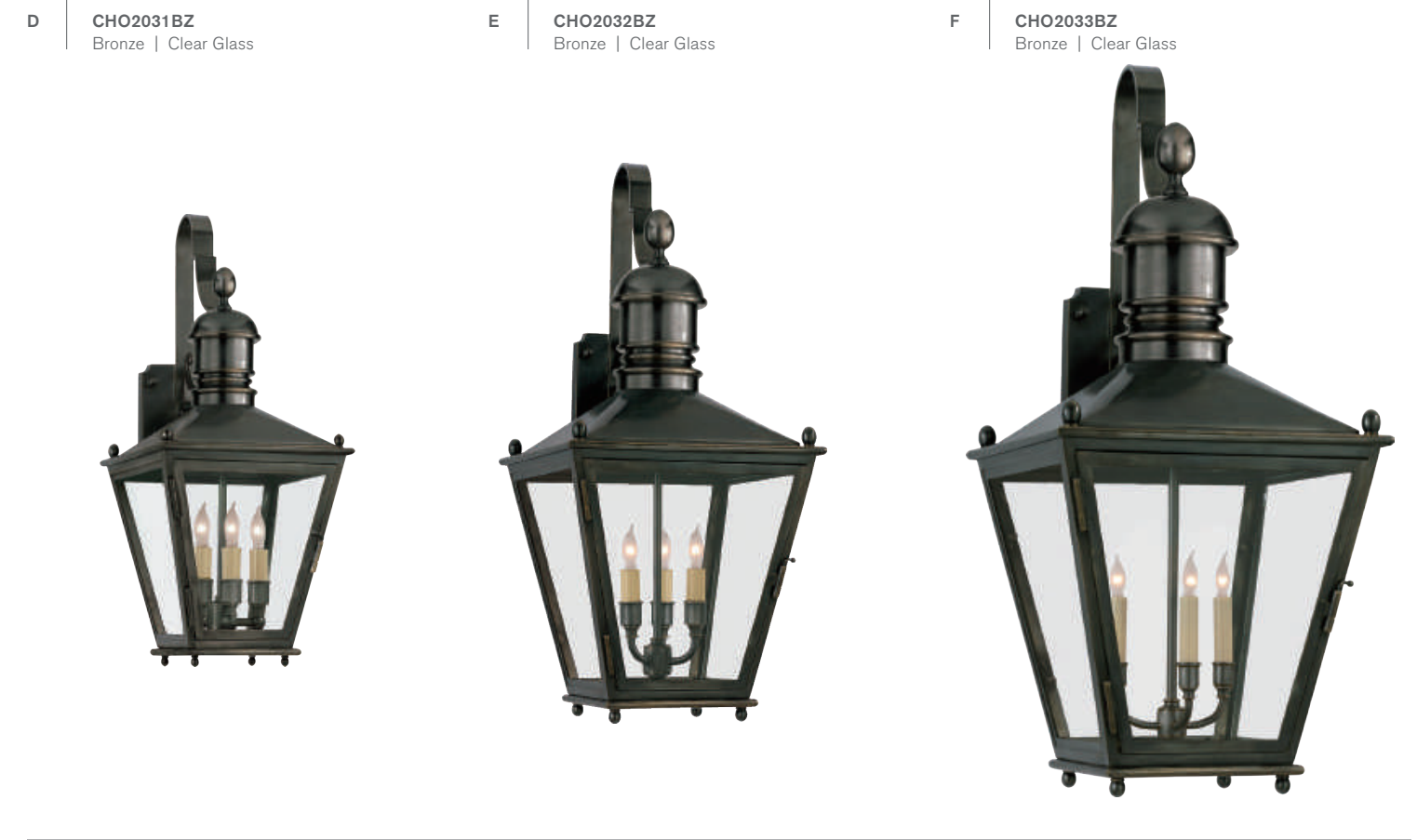
D SUSSEX SMALL BRACKET WALL LANTERN E. F. CHAPMAN CHO2031 H: 22.25" | W: 9.5" | Ext: 11.5" Backplate: 4.5" x 5" Socket: 3 - E12 Candelabra | Bulb: 3 - 60 C ©EFC DESIGNS E SUSSEX MEDIUM BRACKET WALL LANTERN E. F. CHAPMAN CHO2032 H: 27.25" | W: 12.25" | Ext: 13" Backplate: 4.5" x 6" Socket: 3 - E12 Candelabra | Bulb: 3 - 60 C ©EFC DESIGNS F SUSSEX LARGE BRACKET WALL LANTERN E. F. CHAPMAN CHO2033 H: 36" | W: 16" | Ext: 17" Backplate: 7" x 5" Socket: 3 - E12 Candelabra | Bulb: 3 - 60 C ©EFC DESIGNS
