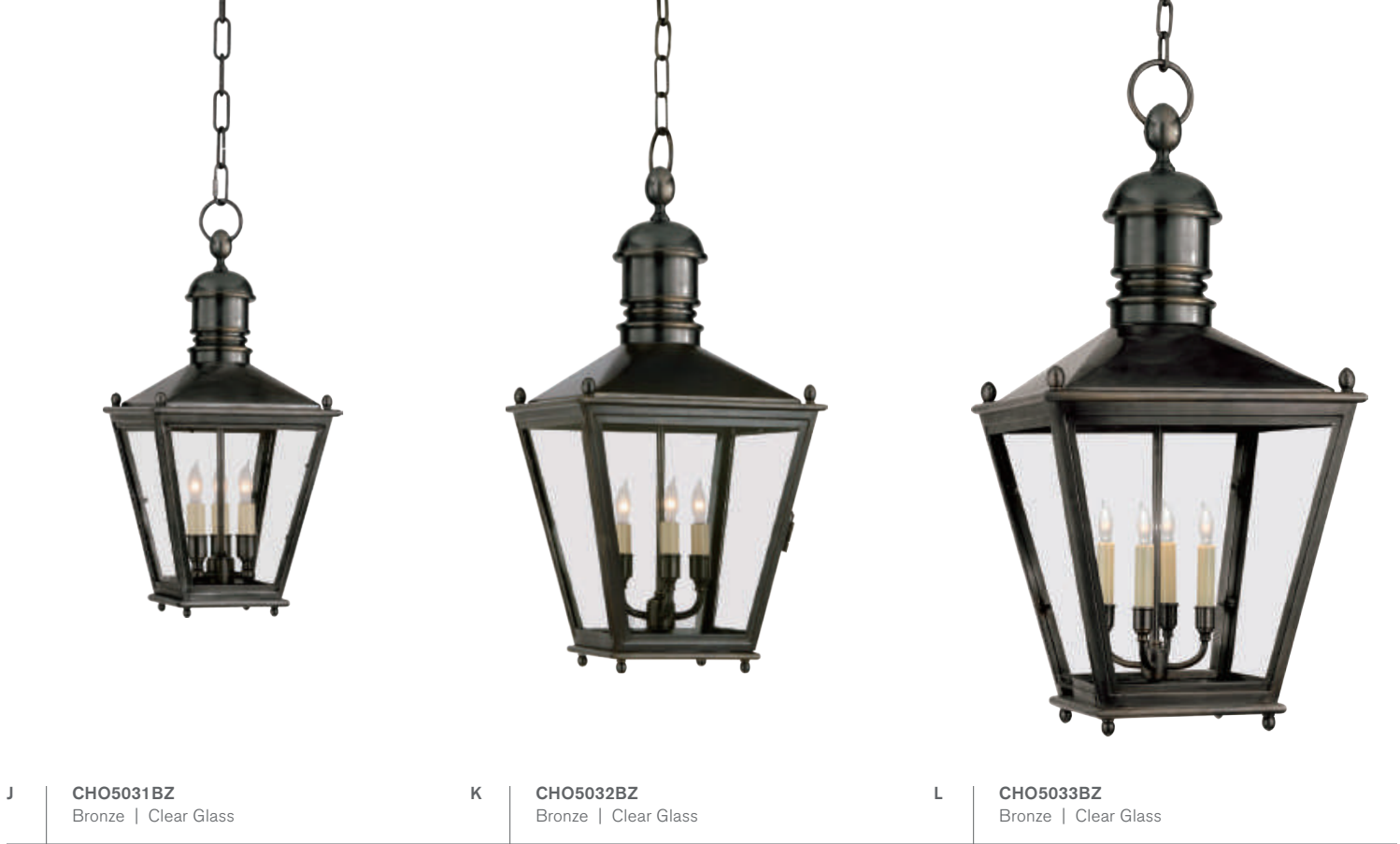
J SUSSEX SMALL HANGING LANTERN E. F. CHAPMAN CHO5031 H: 20.5" | W: 9.5" | Canopy: 5.5" Round Socket: 3 - E12 Candelabra | Bulb: 3 - 60 C ©EFC DESIGNS K SUSSEX MEDIUM HANGING LANTERN E. F. CHAPMAN CHO5032 H: 26" | W: 12.25" | Canopy: 5.5" Round Socket: 3 - E12 Candelabra | Bulb: 3 - 60 C ©EFC DESIGNS L SUSSEX LARGE HANGING LANTERN E. F. CHAPMAN CHO5033 H: 33" | W: 16" | Canopy: 5.5" Round Socket: 4 - E12 Candelabra | Bulb: 4 - 60 C ©EFC DESIGNS
