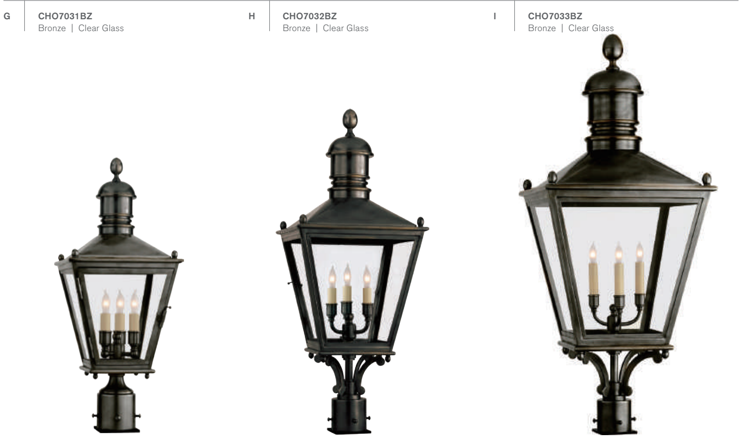
G SUSSEX SMALL POST LANTERN E. F. CHAPMAN CHO7031 H: 23.5" | W: 9.5" | Base: 3" Round Post Cap Socket: 3 - E12 Candelabra | Bulb: 3 - 60 C ©EFC DESIGNS H SUSSEX MEDIUM POST LANTERN E. F. CHAPMAN CHO7032 H: 30.25" | W: 12.25" | Base: 3" Round Post Cap Socket: 3 - E12 Candelabra | Bulb: 3 - 60 C ©EFC DESIGNS I SUSSEX LARGE POST LANTERN E. F. CHAPMAN CHO7033 H: 37.75" | W: 16" | Base: 3" Round Post Cap Socket: 3 - E12 Candelabra | Bulb: 3 - 60 C ©EFC DESIGNS
