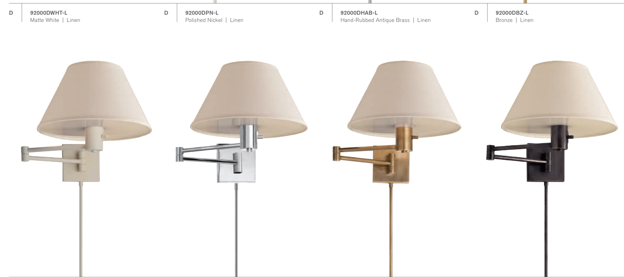
C WALKER SWING ARM SCONCE KATE SPADE NEW YORK KS2075 H: 11.5" | W: 12" | Ext: 16" - 25.25" Backplate: 5" Round Socket: E26 Keyless | Bulb: 60 A Shade: 12" x 12" x 6.5" D CLASSIC SWING ARM SCONCE STUDIO VC 92000D H: 11" | W: 12" | Ext: 25" Backplate: 4.5" Square Socket: E26 Dimmer | Bulb: 75 A Shade: 6" x 12" x 7" Additional Options: Antique Nickel | Linen (AN-L) * Cord Cover Included C KS2075LC-NL Light Cream | Natural Linen C KS2075BSL-L Burnished Silver Leaf | Cream Linen C KS2075G-L/BL Gild | Cream Linen | Black Linen
