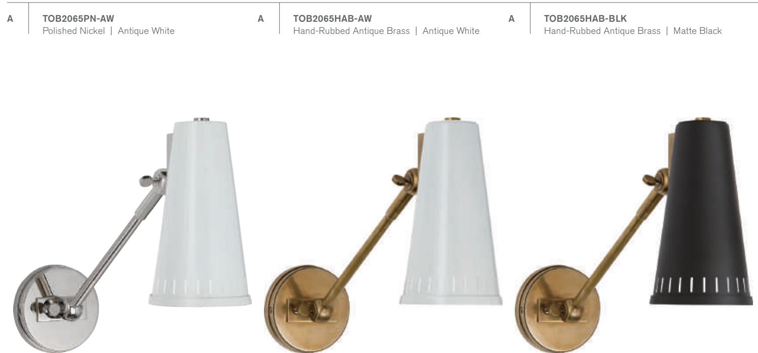
A ANTONIO SINGLE SCENCE THOMAS O'BRIEN TOB2065 H: 8.25" | W: 4.5" | Ext: 7" - 17.75" Backplate: 4.5" Round Socket: E26 Keyless | Bulb: 60 A
